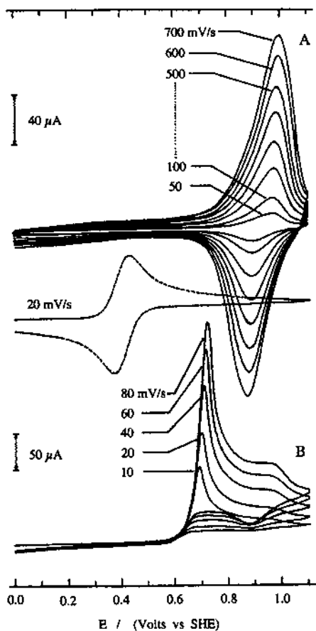
Fig. 12. (A) Cyclic voltammograms of [Ni-TRP](TFMS) 4 film on glassy carbon electrode surface, \Gamma_T = 1.0 \text{ nmol cm}^{-2} ; in LiTFMS 0.25 M, acetate buffer 0.05 M, pH 4.7. (B) Cyclic voltammograms of K 4 [Fe(CN) 6 ] 5.37 mM in bare electrode (top) and on Ni-TRP modified glassy carbon, \Gamma_T = 0.74 \text{ nmol cm}^{-2} (bottom).
