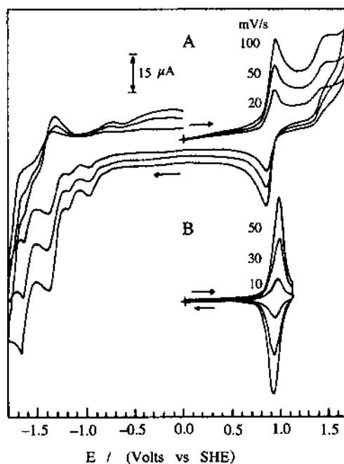
Fig. 7. (A) Cyclic voltammograms of [Zn–TRP](TFMS) 4 ( 9.9 \times 10^{-4} M) in DMF (0.10 M TEAClO 4 ) obtained using a platinum disc electrode. (B) CV of a 1.8 \times 10^{-8} mol cm -2 film adsorbed on a glassy carbon disc electrode, in 0.026 M acetate buffer (pH 4.7) and 0.25 M LiTFMS.
