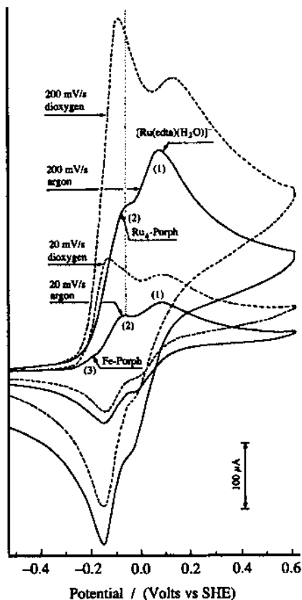
Fig. 2. Cyclic voltammograms of the [Fe III TPyP{Ru III (edta)} 4 ] complex, 1.8 \times 10^{-3} mol dm -3 , in argon or dioxygen saturated solutions, showing the catalytic peak at -0.1 V. [Ru(edta)(H 2 O)] = 1.8 \times 10^{-3} mol dm -3 , [KCl] = 0.50 mol dm -3 , pH 4.5 (acetate buffer, 0.05 mol dm -3 ), glassy carbon electrode, 25°C.
