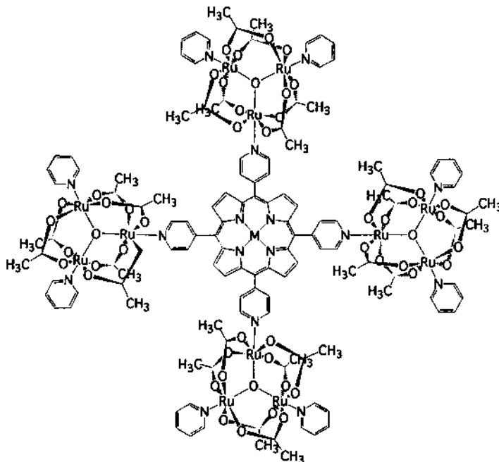
Fig. 17. Structural representation of the tetracluster porphyrin (TCP) supermolecule.
