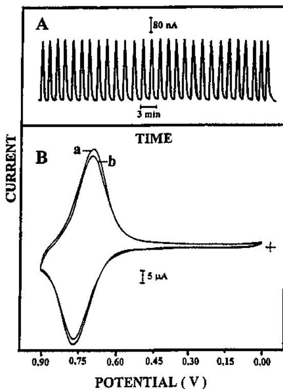
Fig. 16. (A) FIA amperometric responses to consecutive 100 \mu\text{l} injections of nitrite ( 10^{-5} \text{ mol dm}^{-3} ) and (B) cyclic voltammograms of a glassy carbon electrode modified with [\text{CoTRP}]/[\text{ZnTPPS}] bilayered film in the presence of the carrier solution (a) before and (b) after 1 h of continuous nitrite analysis by FIA. Conditions for FIA: E = +0.90 V, flow rate = 0.8 \text{ cm}^3 \text{ min}^{-1} ; cyclic voltammetry scan rate = 100 \text{ mV s}^{-1} .
