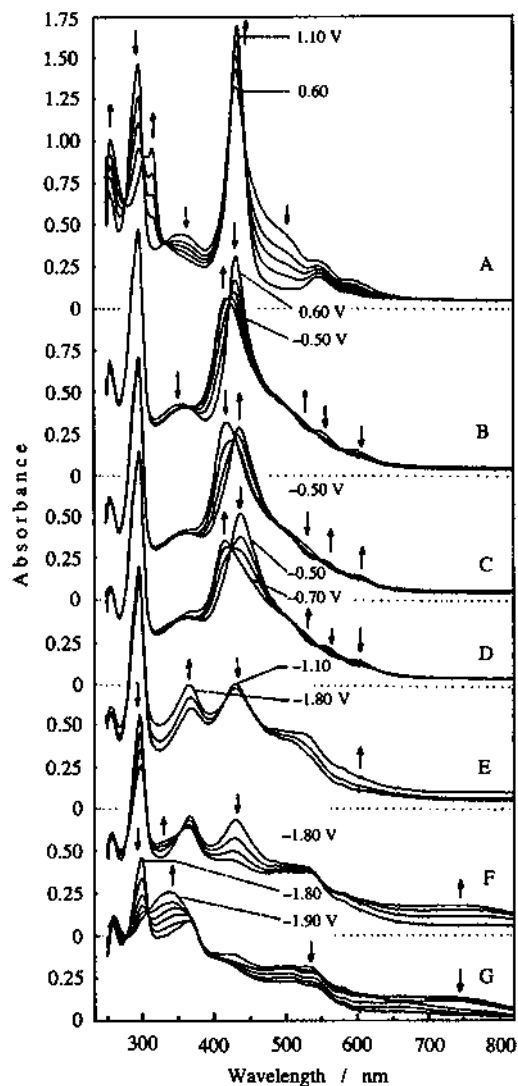
Fig. 9. Spectroelectrochemistry of 1 mM [\text{CoTRP}](\text{TFMS})_4 in DMF solution containing 0.10 M \text{TEAPF}_6 in the potential range 1.10 to -1.90 V vs. SHE.
