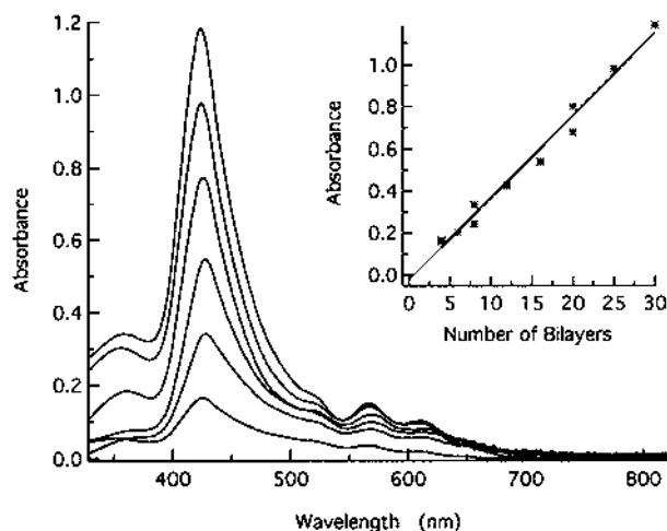
Fig. 15. UV–vis spectra of 4, 8, 16, 20, 25 and 30 bilayer films of [Zn–TRP]/[TPPS] on ITO. Inset: growth of the absorbance as a function of the number of bilayers.
